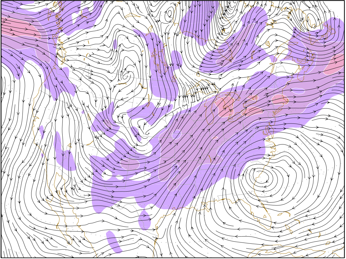
700mb Streamlines (solid black) and Wind Speed (shaded)
