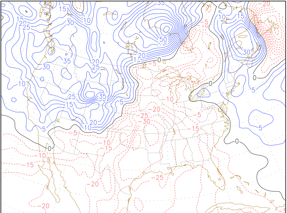
700mb Geopotential Height Change Over 6 Hours
